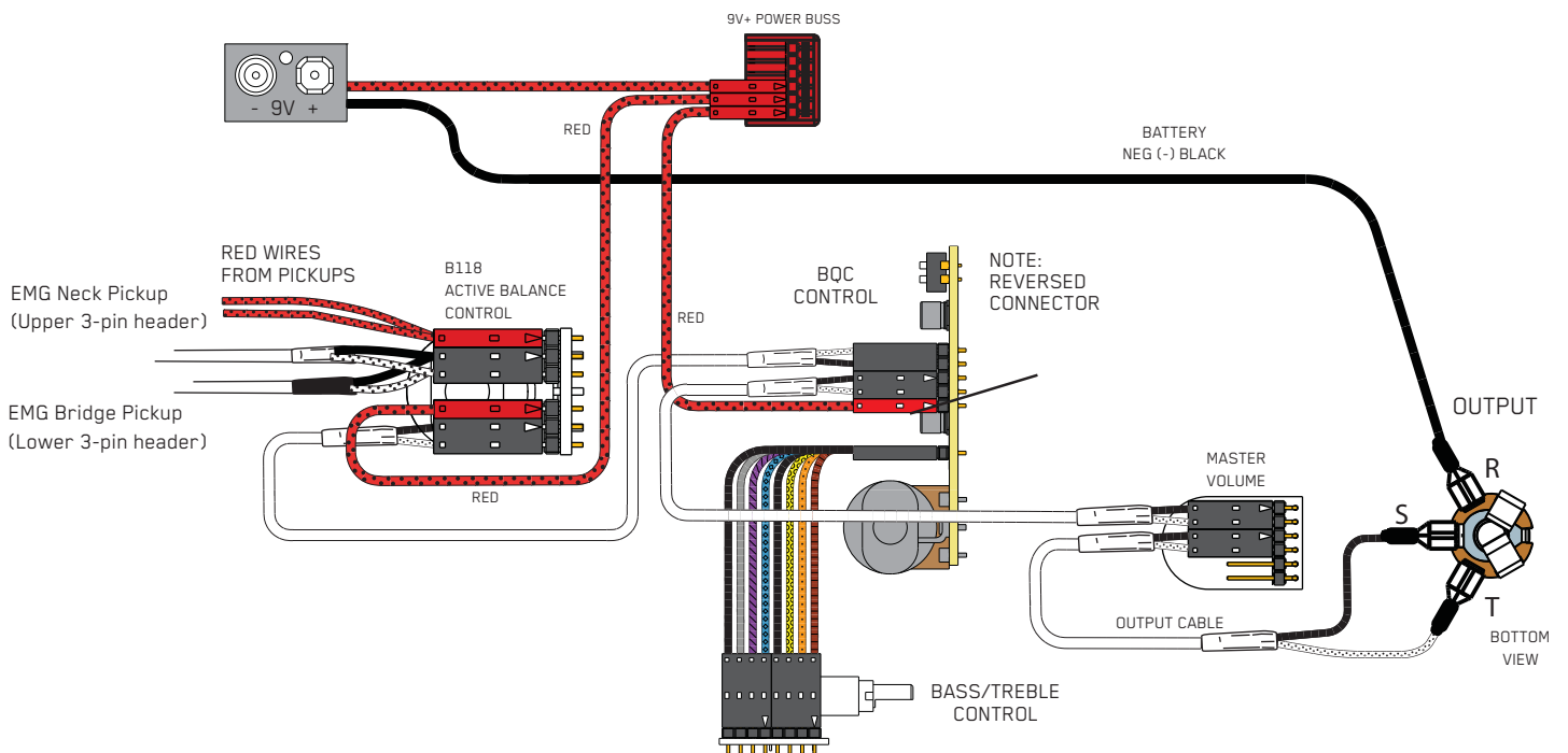
Diagram #3 (preferred wiring order) ABC Control BQC Control Master Volume Output Jack
