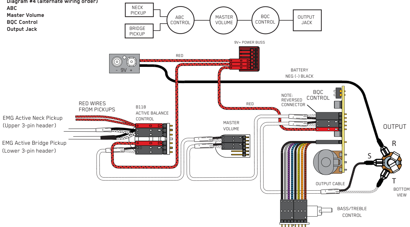
Diagram #4 (alternate wiring order)
